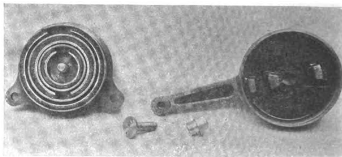
Sphinx Shock Absorber Dismounted to Show Parts
